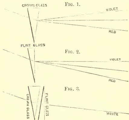
Refraction and Dispersion by Prisms.
